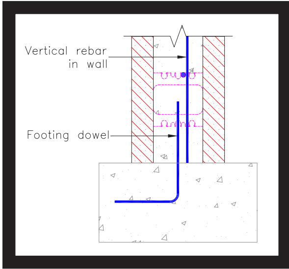
Figure 4: Wall/Footing connection
